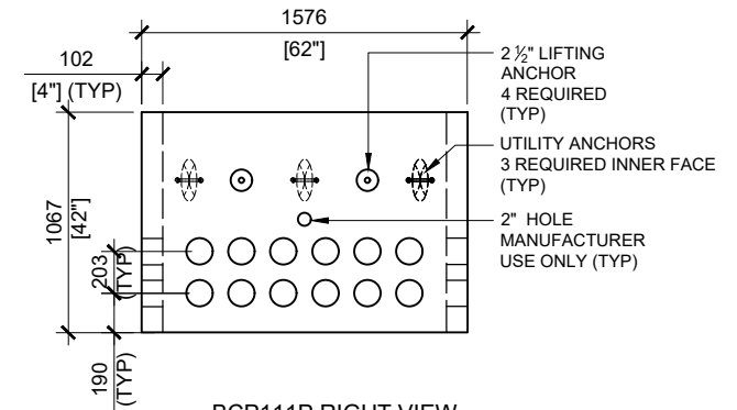
BCP111P RIGHT VIEW SCALE: 1/40
