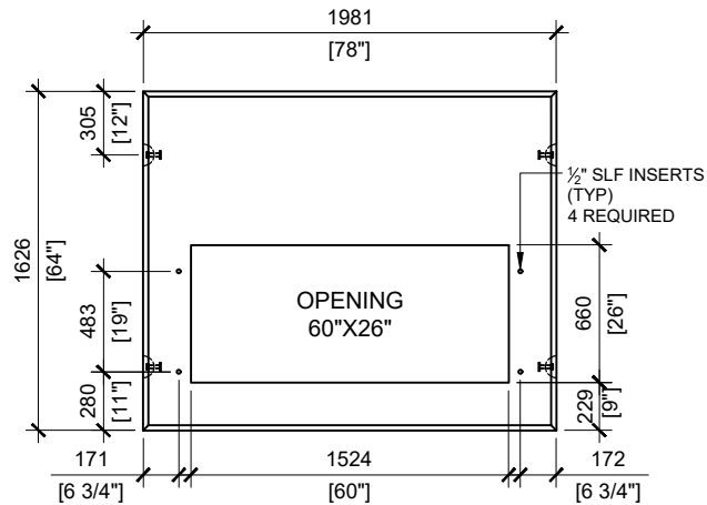
BCP111THO3 TOP VIEW SCALE: 1/40
