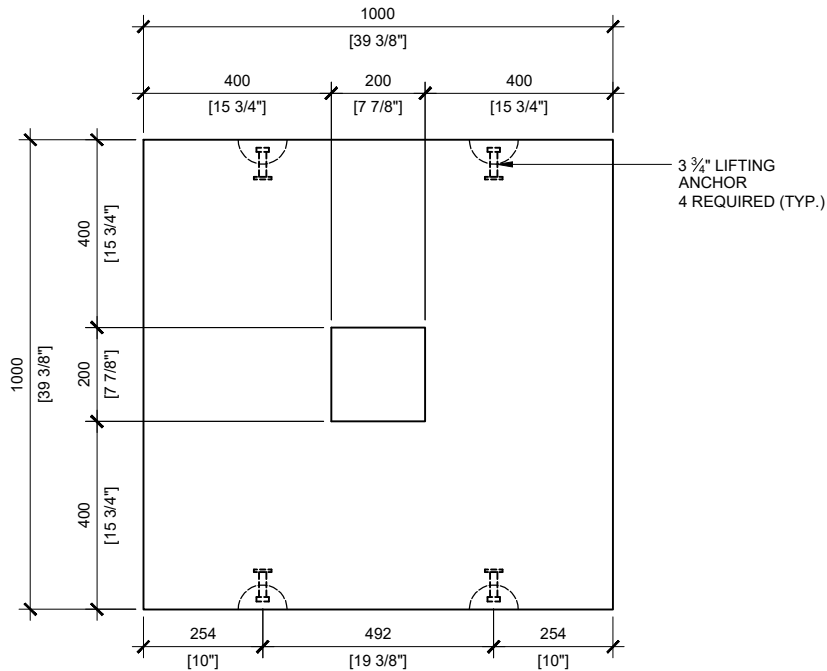
TOP VIEW SCALE: 1/16
