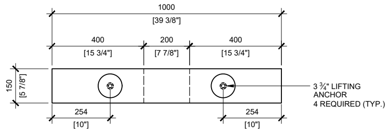
FRONT VIEW SCALE: 1/16
