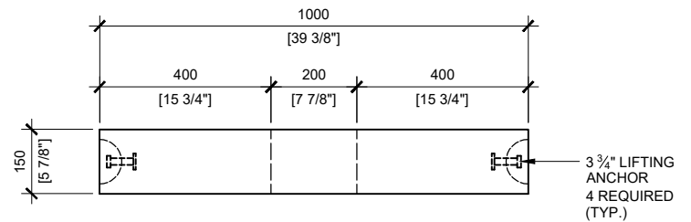
RIGHT VIEW SCALE: 1/16
