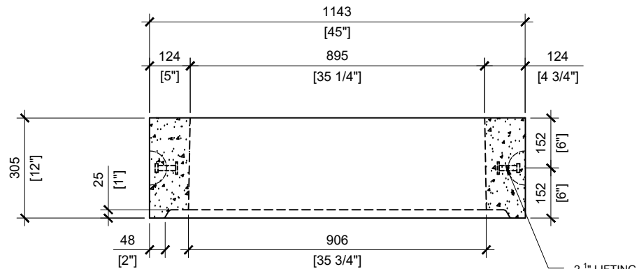
12" RISER FRONT VIEW SCALE: 1/16
