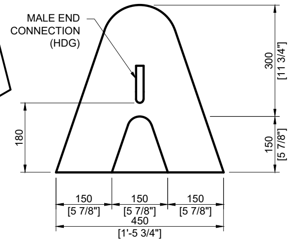
LEFT VIEW SCALE 1/10
